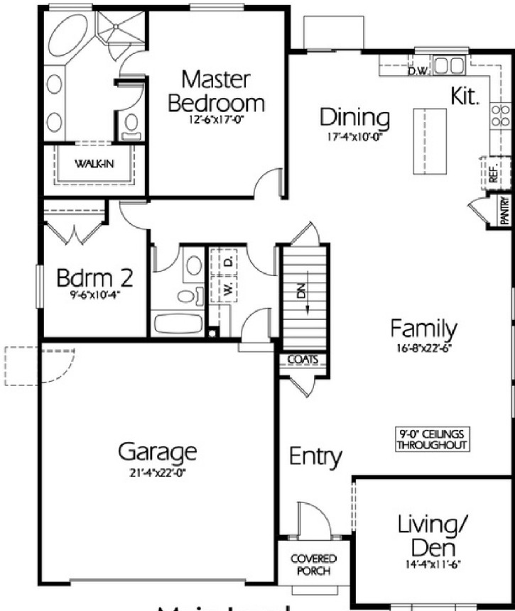
Main Level 1783 Sq. Feet
